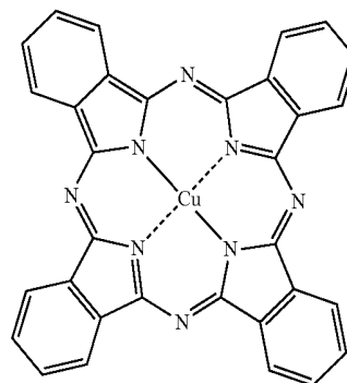
CuPc
