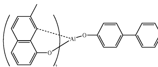
BAQ
